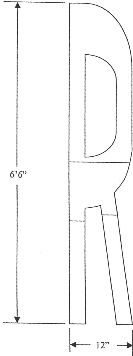
6'6" "R" FHWA
