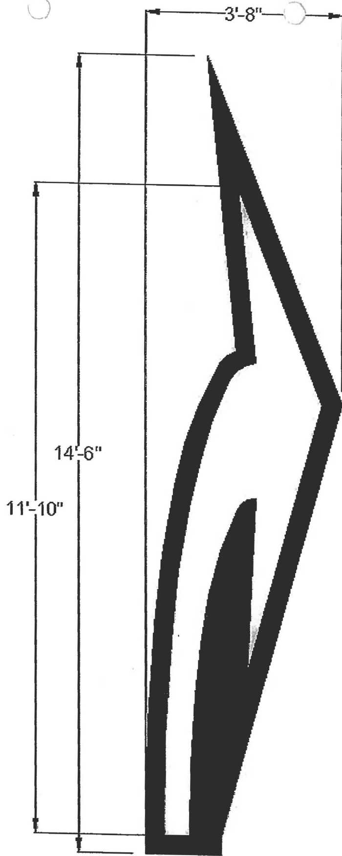
12' Right Turn Arrow w/4" contrast
